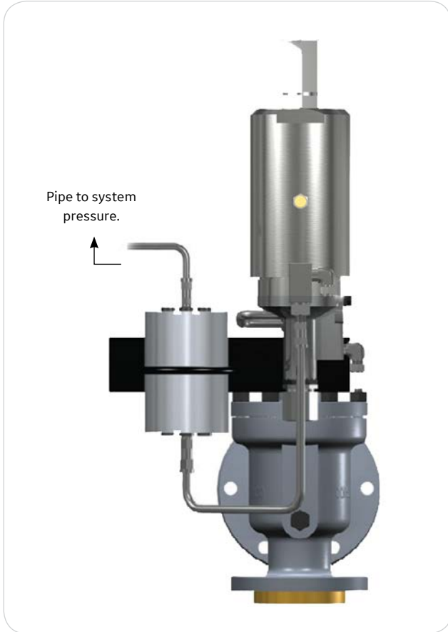
Heat Exchanger with Remote Sensing (Standard) (High Temperature Configuration)
