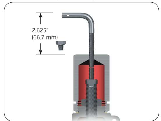
1982 Series Cap with Gag
