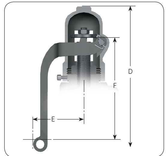
1982 Series Plain Lever
