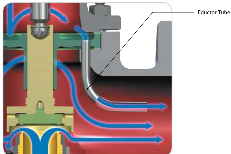
Eductor Tube
